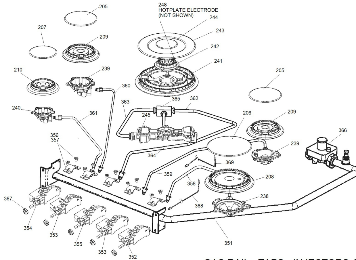
GAS RAIL - TAPS - INJECTORS AND PIPES
